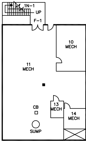
BASEMENT GROSS AREA = 3,177 S.F.
