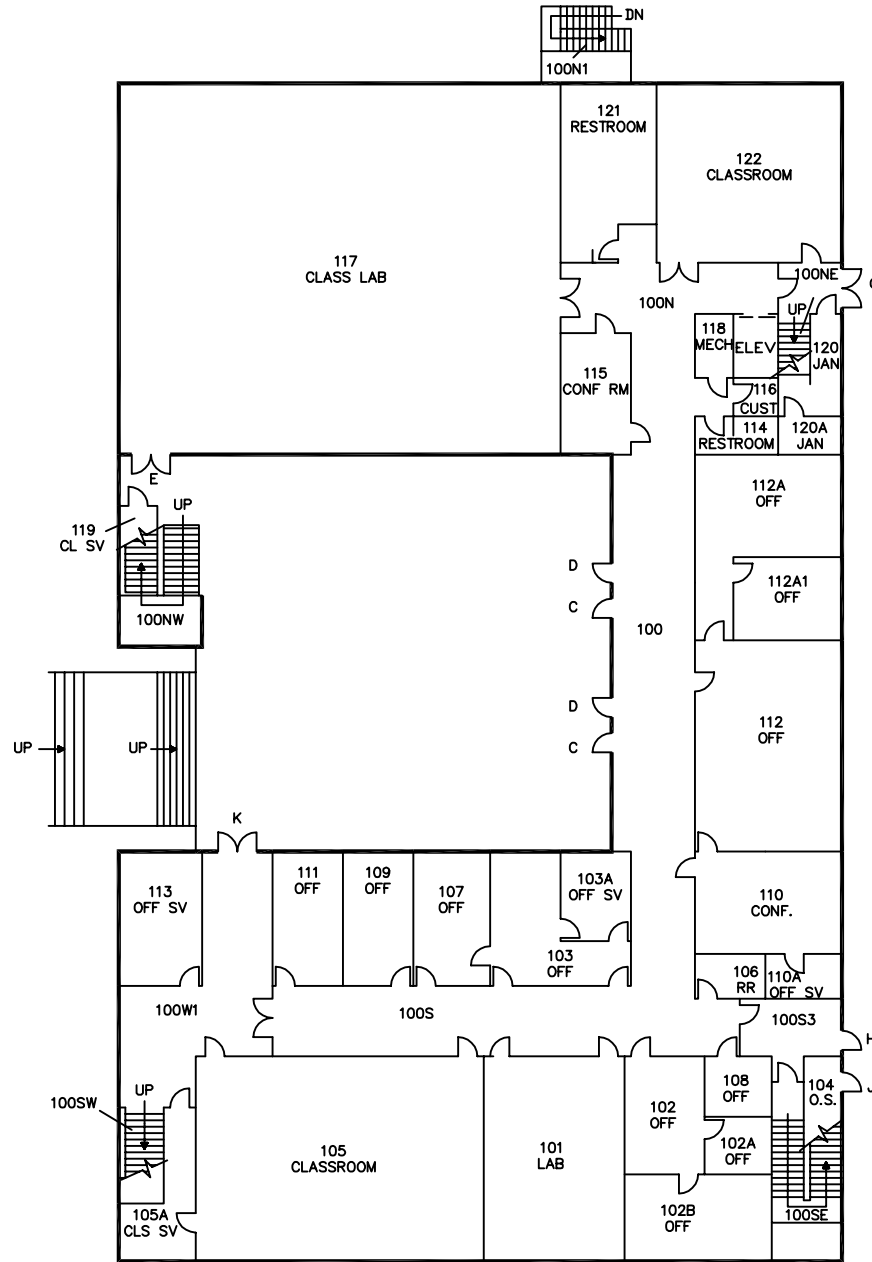
FIRST FLOOR GROSS AREA = 16,018 S.F.
